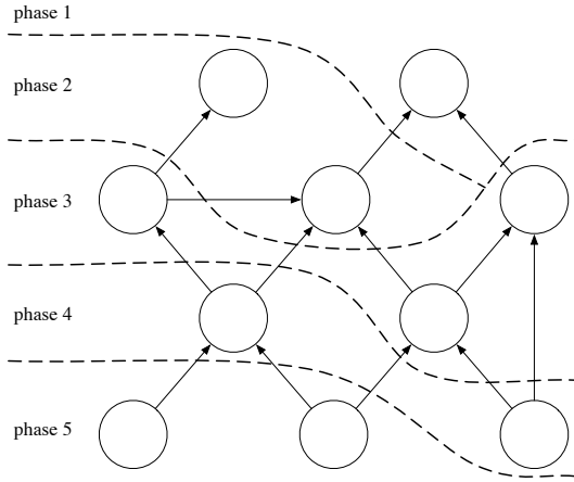
Figure 1. A 10-node graph in which 5 phases are being executed concurrently.
